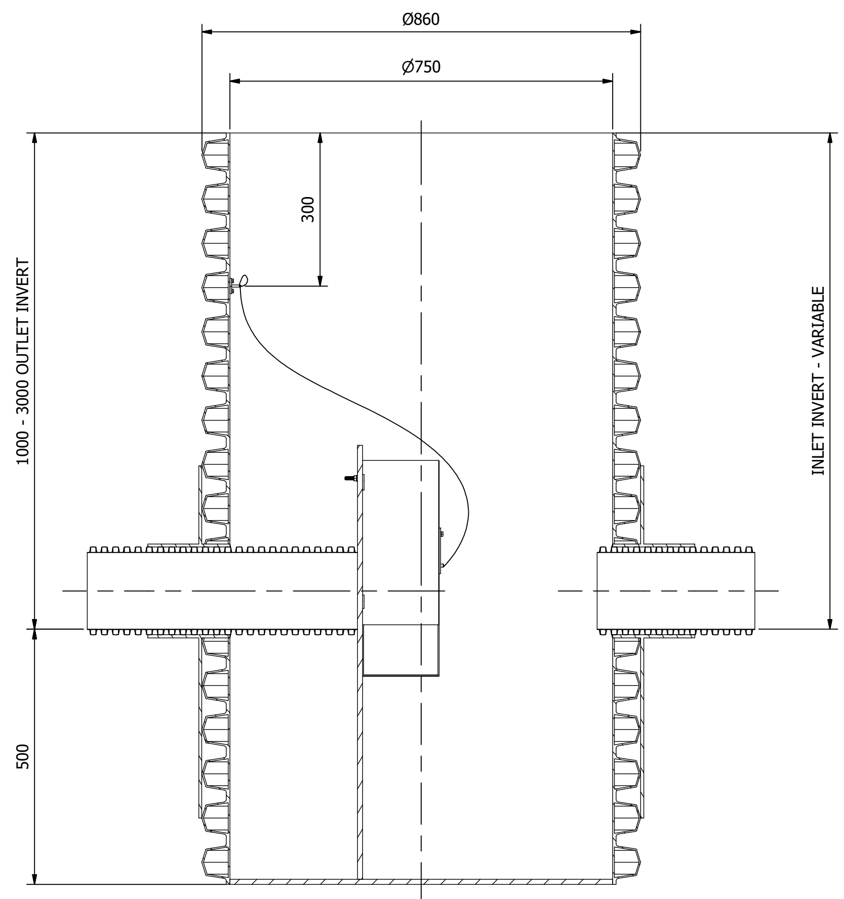
SECTION A-A SCALE 1:7.5
